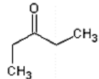
pentan-3-one
